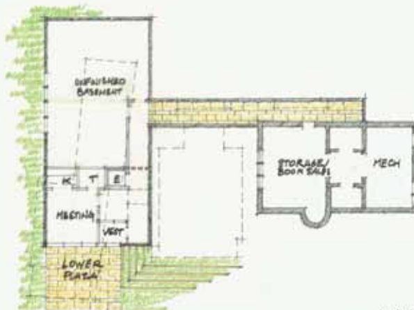
Jeudevine Memorial Library Scale 1/4"=1'-0" July 2016
